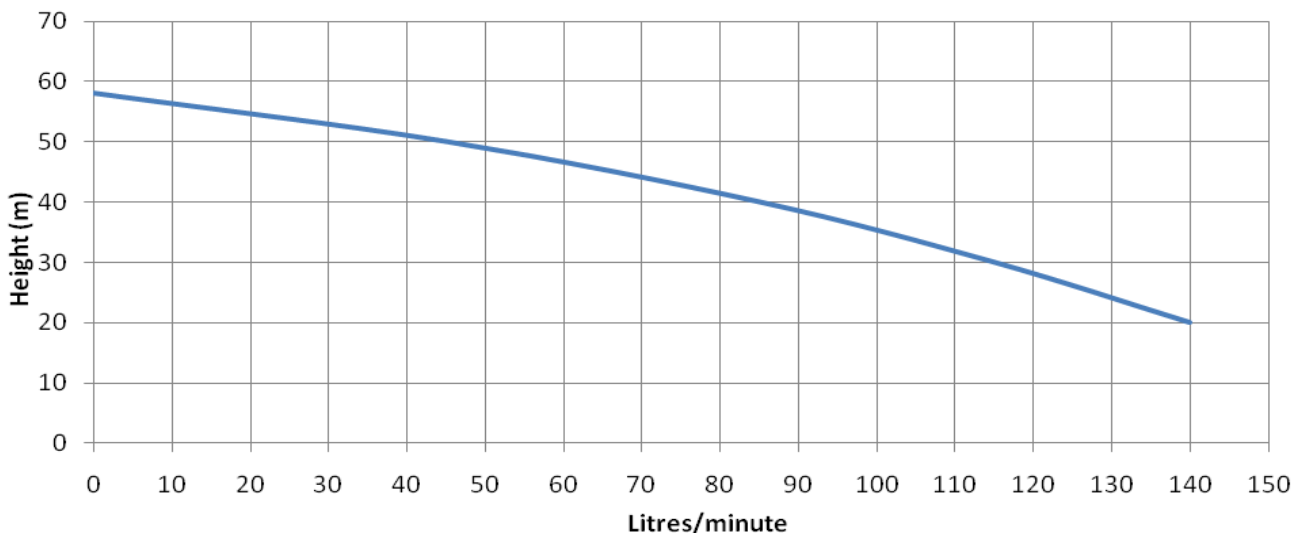
Pump Performance
